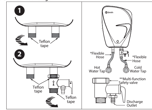
Figure 10 Installation Diagram
